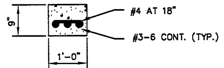
FOOTING DETAIL
