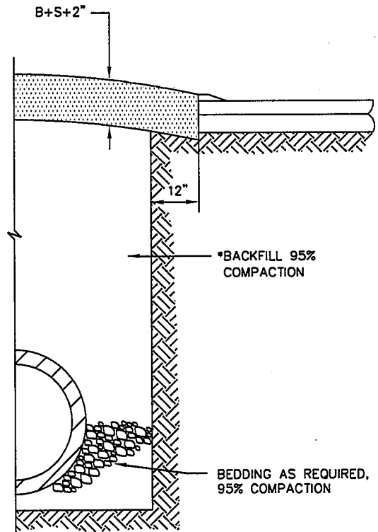
TYPICAL VERTICAL TRENCH
