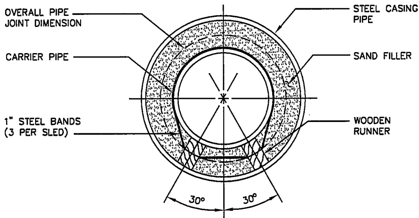
PIPE CASING DETAIL
