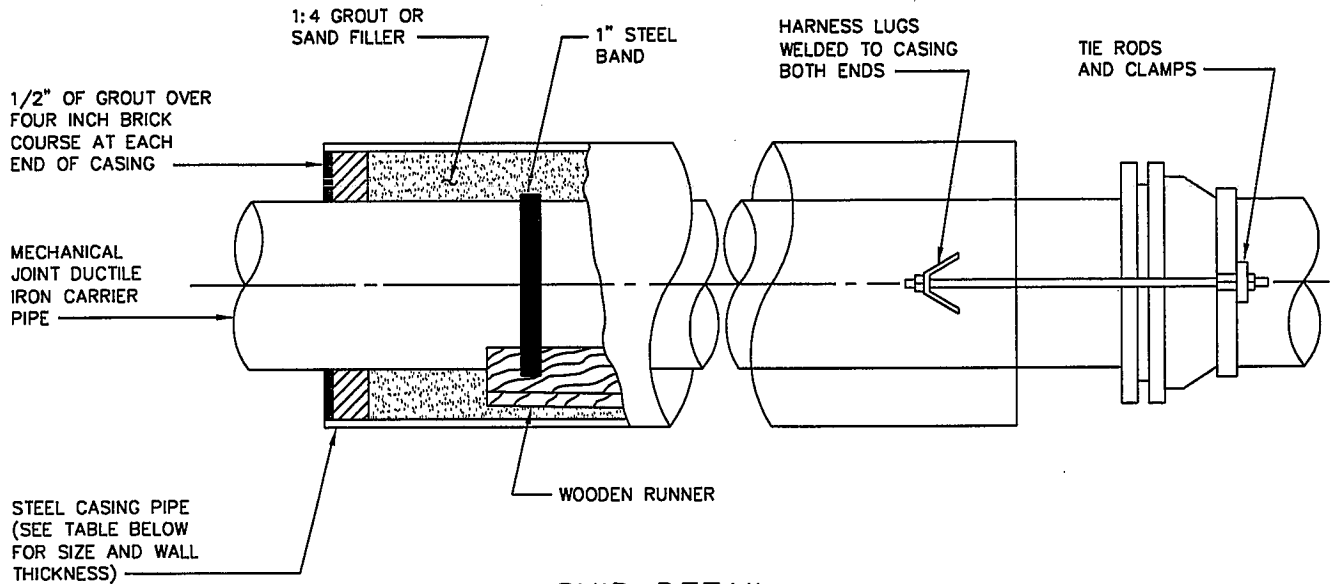
SKID DETAIL
