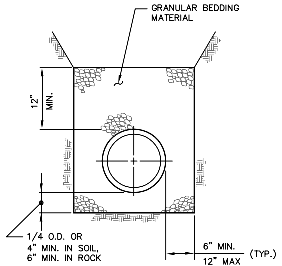
CLASS B ALTERNATIVE COMPACTED GRANULAR BEDDING
