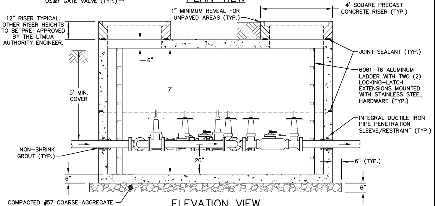
ELEVATION VIEW
